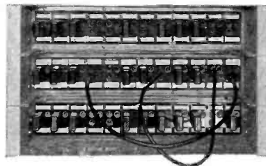
Video Jack Panel, MI-26245. For patching video and/or sync signals. Includes 12 groups of coaxial jack assemblies (3 per group). Video jack plugs and cords, extra.
